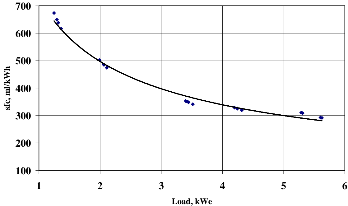
Fig. 5: Specific Fuel Consumption against Load in Diesel Mode
