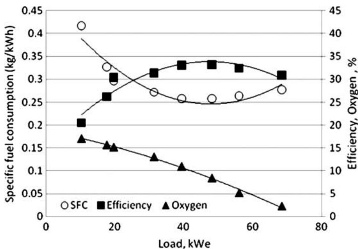
Figure 2. Performance of the engine with diesel alone as fuel.
