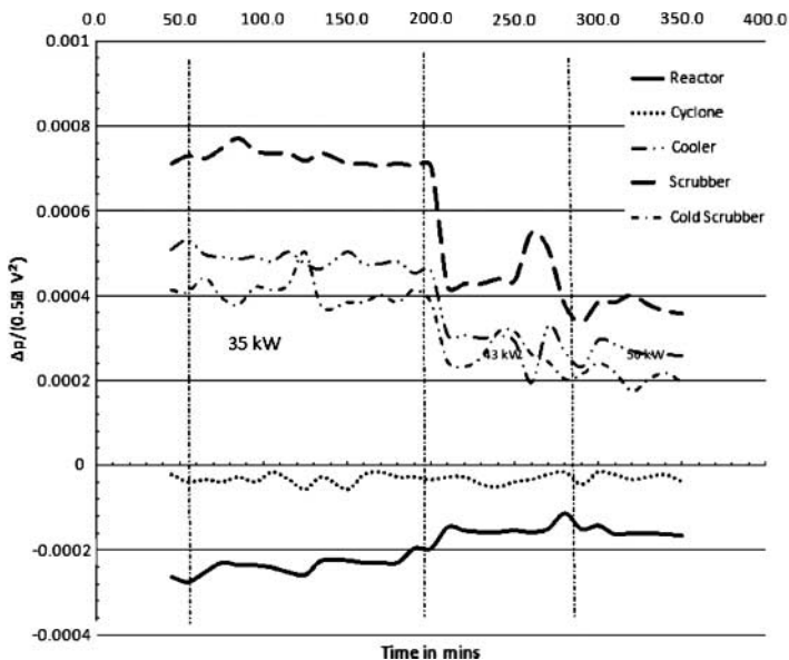
Figure 3. Normalized pressure drop across various elements in the gasifier system.
