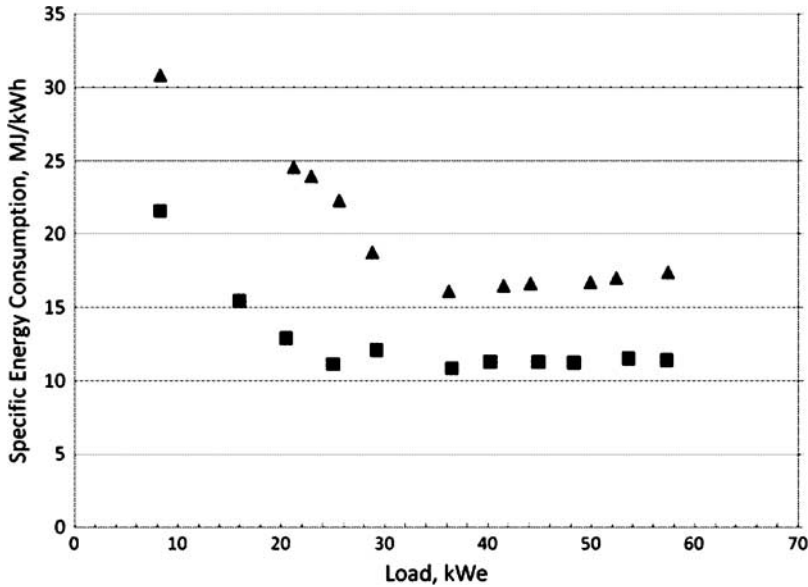
Figure 5. SEC in diesel and dual fuel modes.
