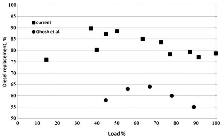
Figure 6. Comparison of diesel replacement with load.
