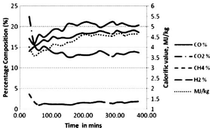
Figure 4. Gas composition and calorific value during a typical dual fuel operation.
