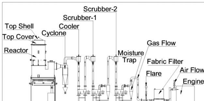
Figure 1. Schematic of the gasification system.
